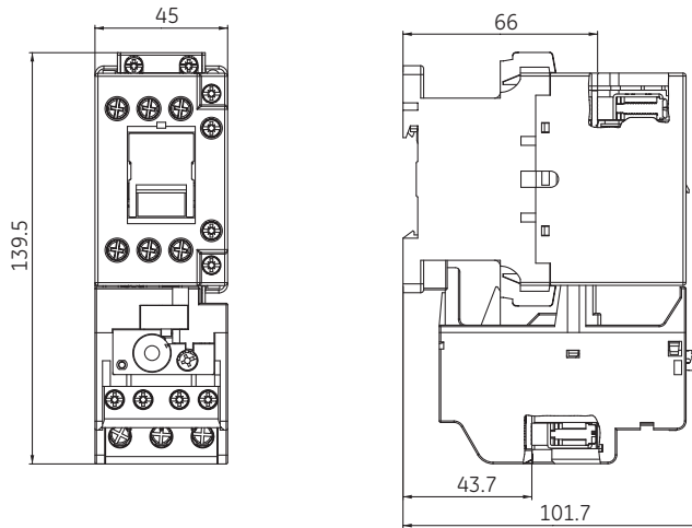
Combination of contactor EC25A and EC25E and thermal overload relay ECRT2
