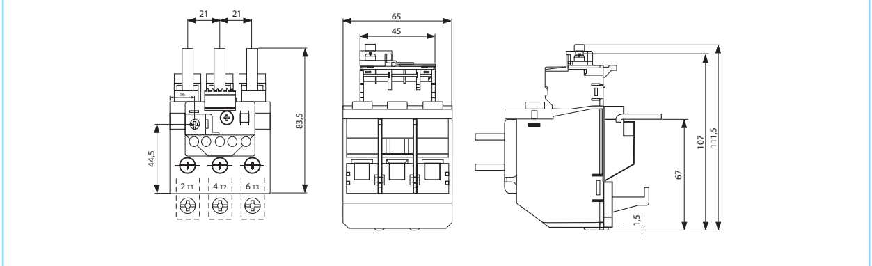
Electronic overload relay RE2 320 g
