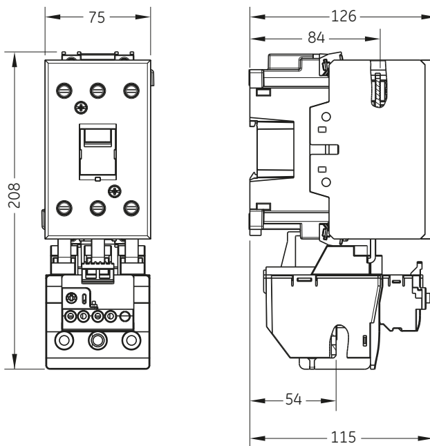
Combination of contactor EF95A3-105A3 and overload relay RE2
