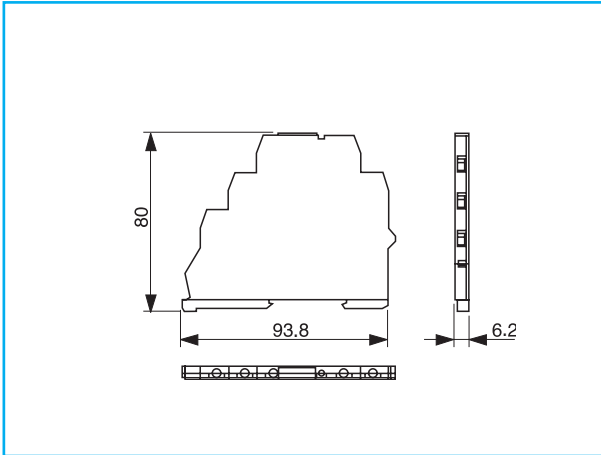
Interface relay
