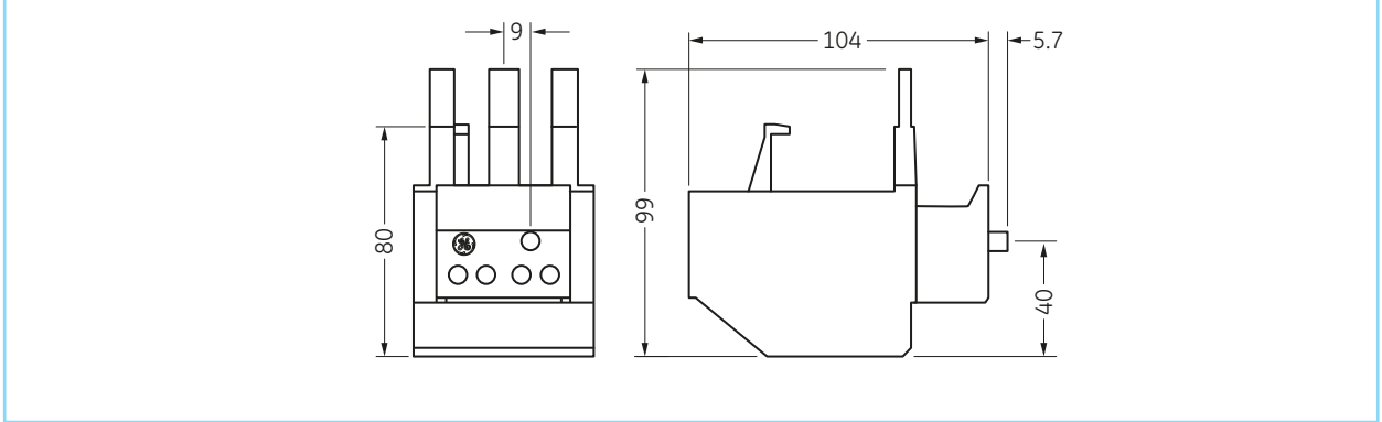
Thermal overload relay RT2 400 g
