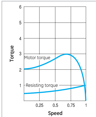
Torque-speed curve
