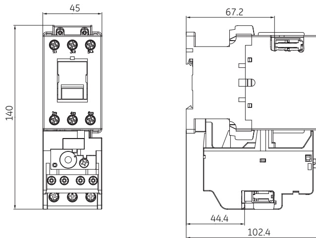
Combination of contactor EC32-40 (A and E) and thermal overload relay ECRT2
