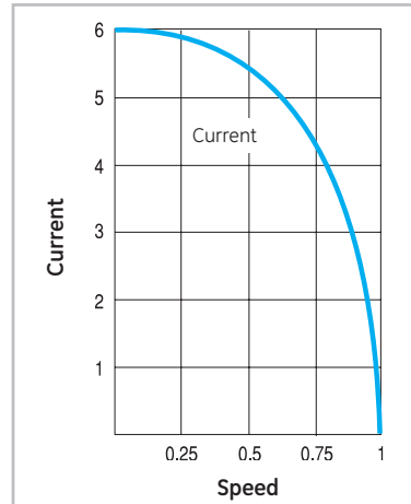
Current-speed curve
