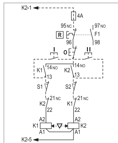
Control circuit
