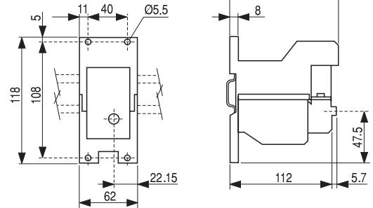
RT2 + RT XP RT22 + RTXP
